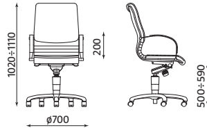
ARTUS-LB MPD170
